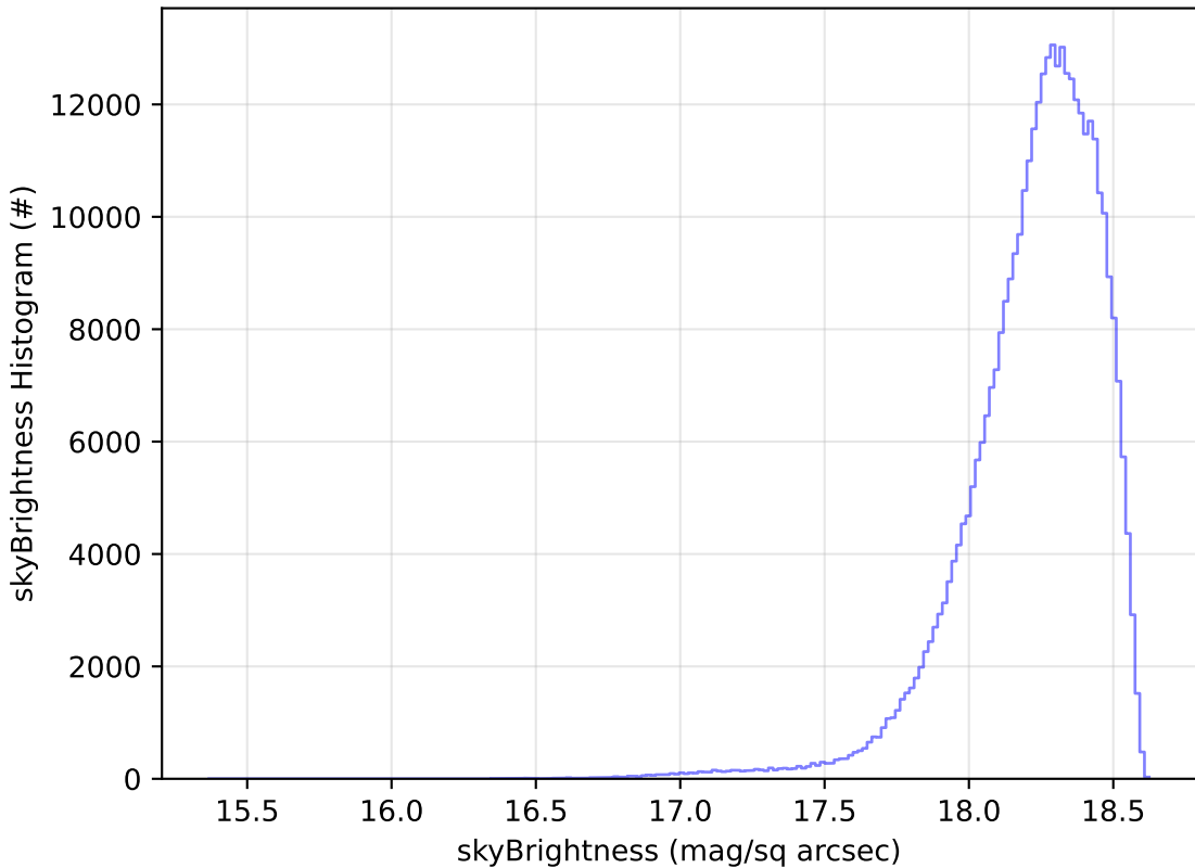
too_5_4v3.4_10yrs All sky y band: skyBrightness Histogram
