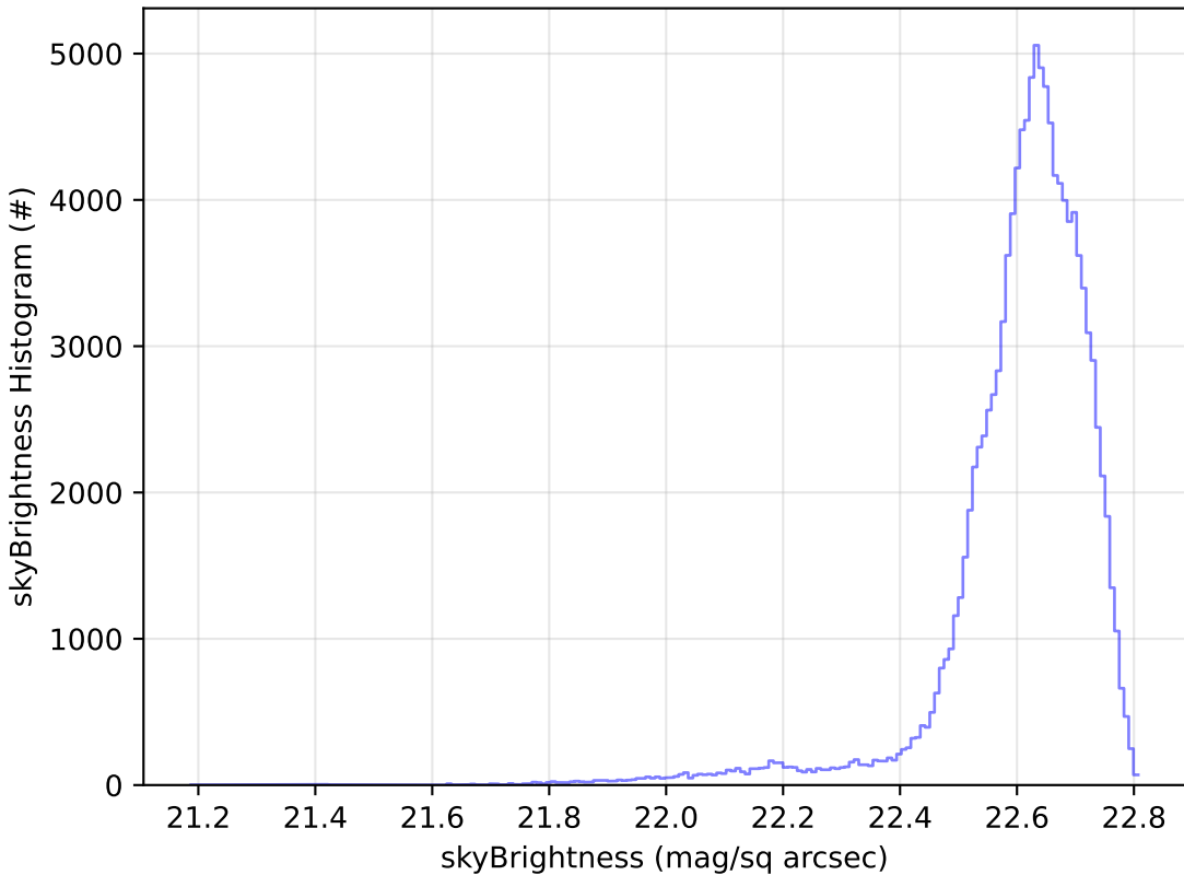
too_5_4v3.4_10yrs All sky u band: skyBrightness Histogram
