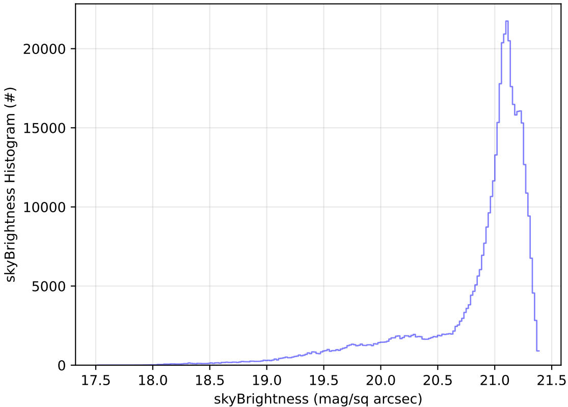
too_5_4v3.4_10yrs All sky r band: skyBrightness Histogram
