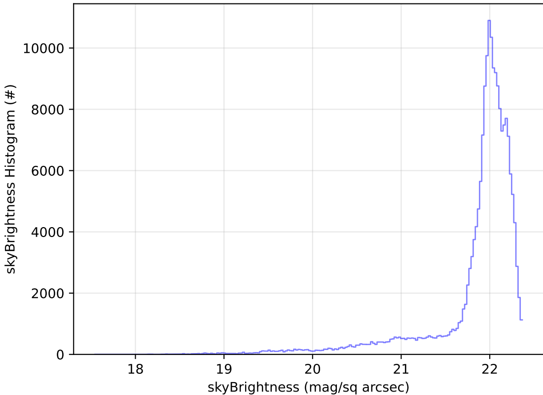
too_5_4v3.4_10yrs All sky g band: skyBrightness Histogram
