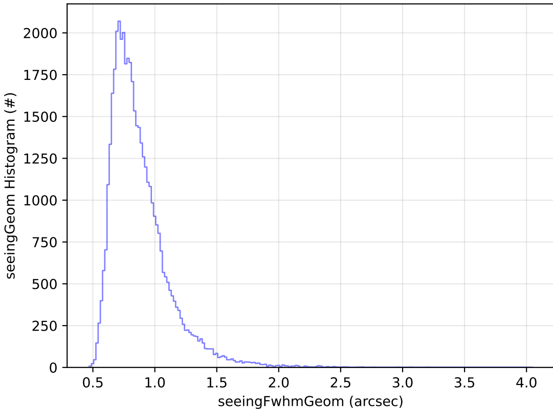
too_5_4v3.4_10yrs Yr 1 z band: seeingGeom Histogram
