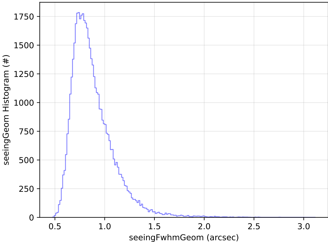
too_5_4v3.4_10yrs Yr 1 y band: seeingGeom Histogram
