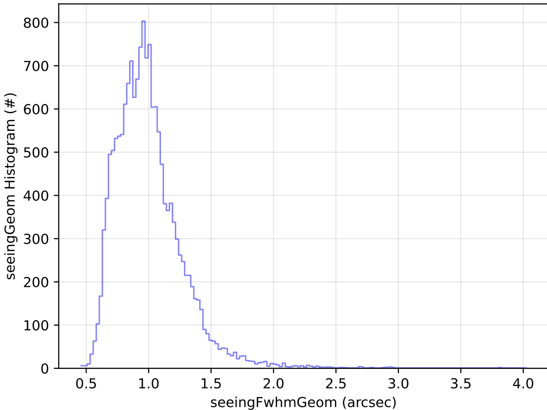
too_5_4v3.4_10yrs Yr 1 u band: seeingGeom Histogram
