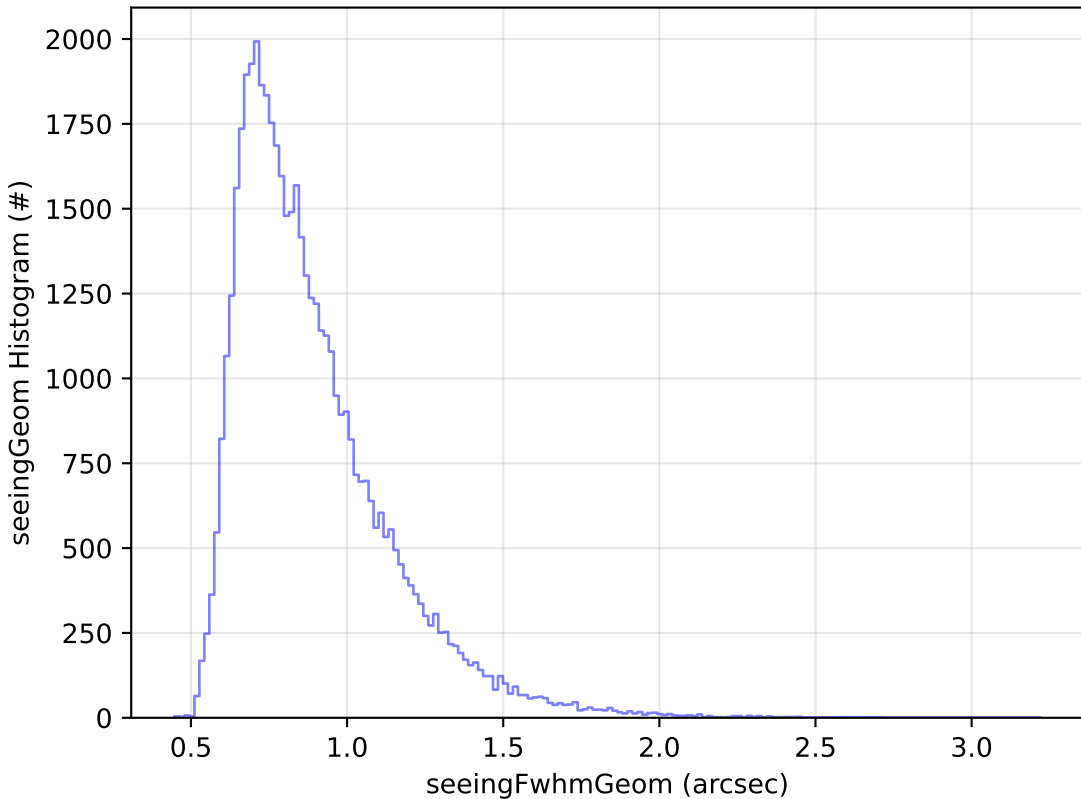
too_5_4v3.4_10yrs Yr 1 r band: seeingGeom Histogram
