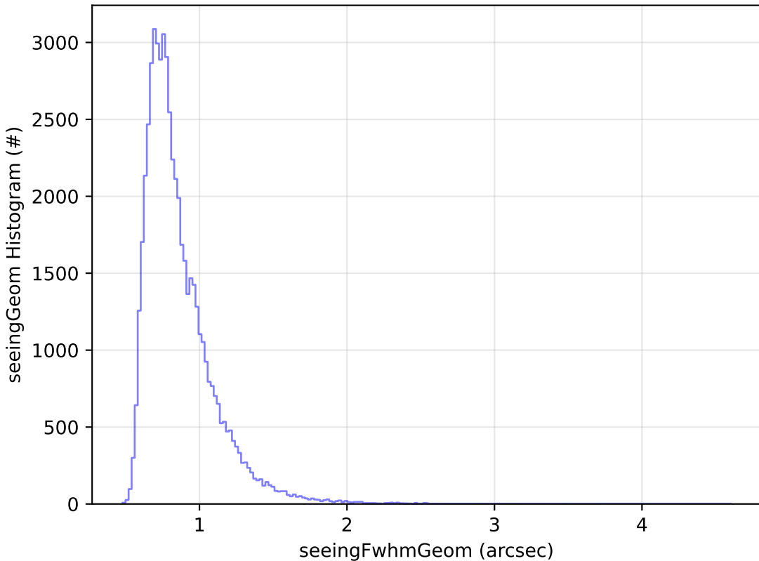
too_5_4v3.4_10yrs Yr 1 i band: seeingGeom Histogram
