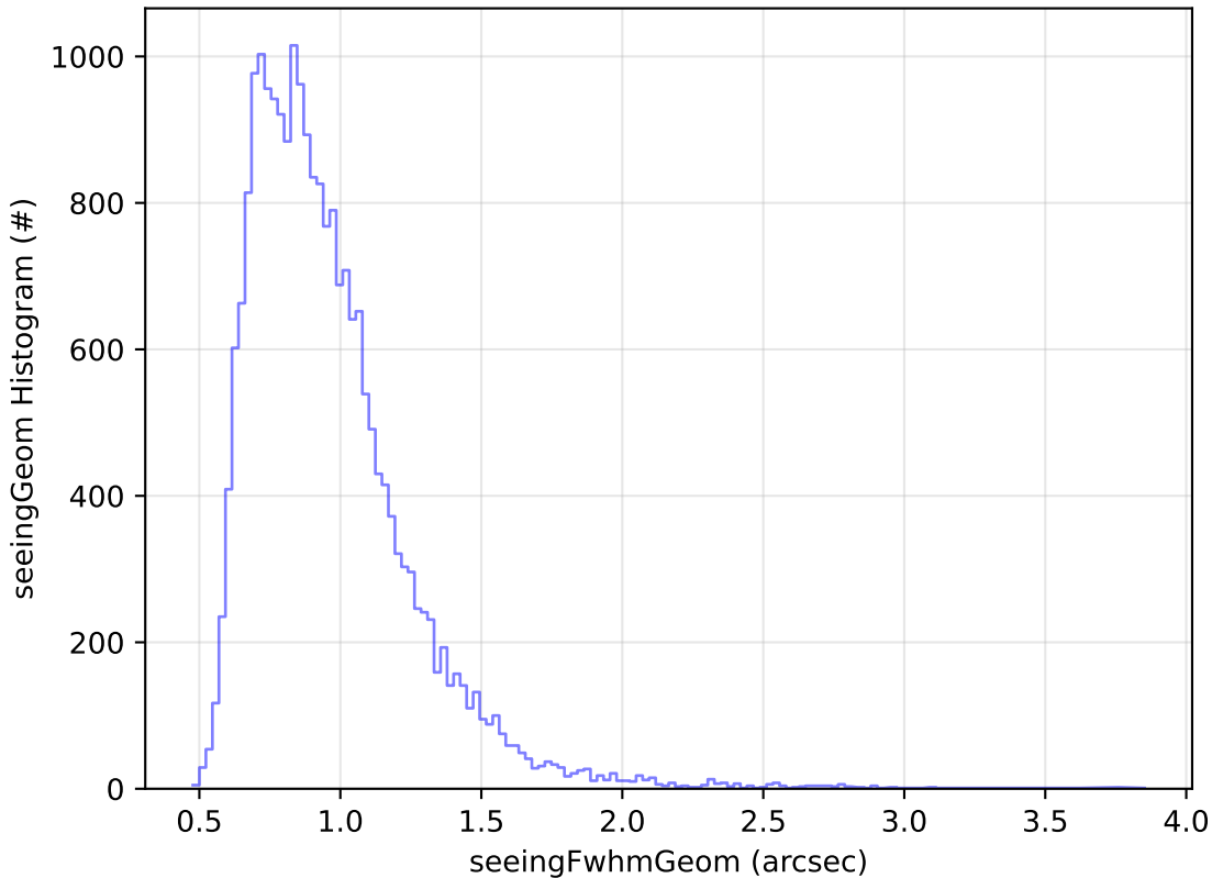
too_5_4v3.4_10yrs Yr 1 g band: seeingGeom Histogram
