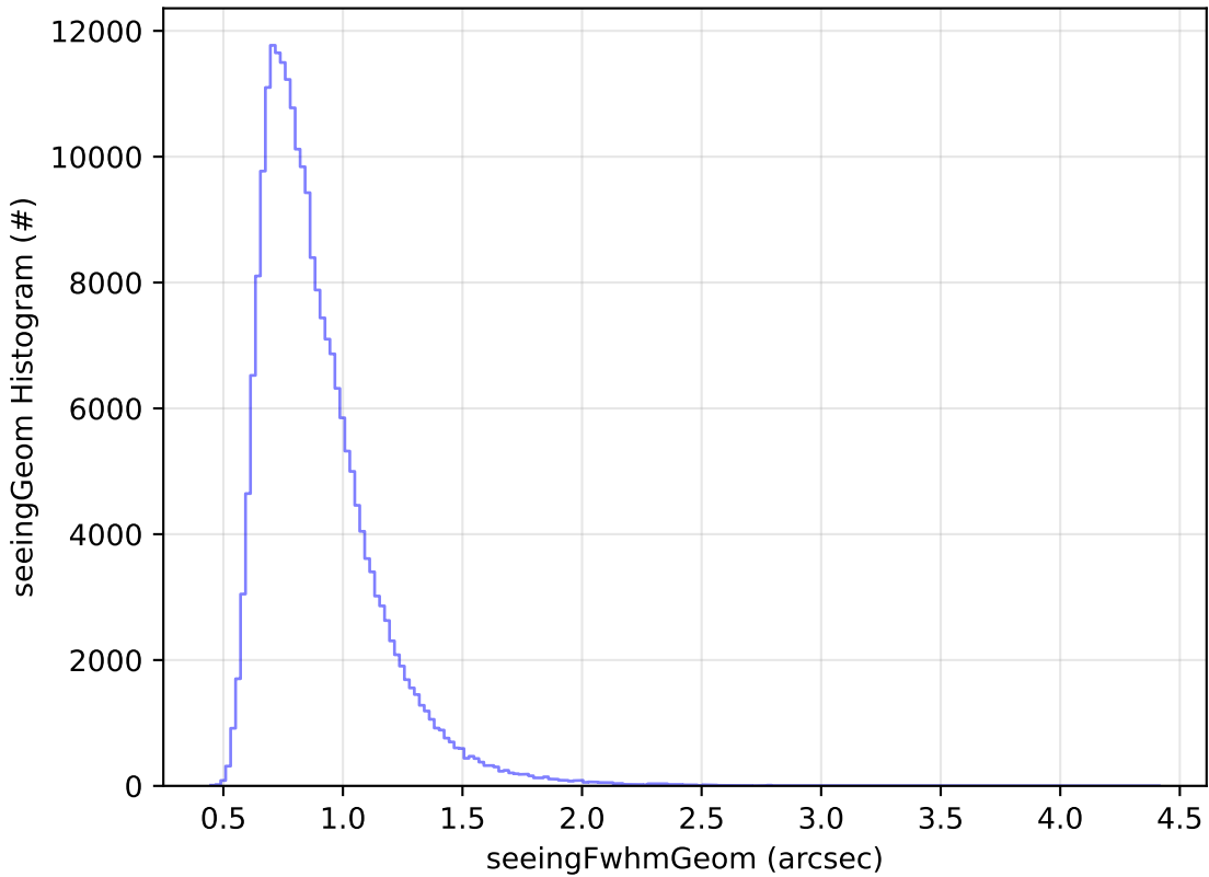
too_5_4v3.4_10yrs Yr 1 all bands: seeingGeom Histogram
