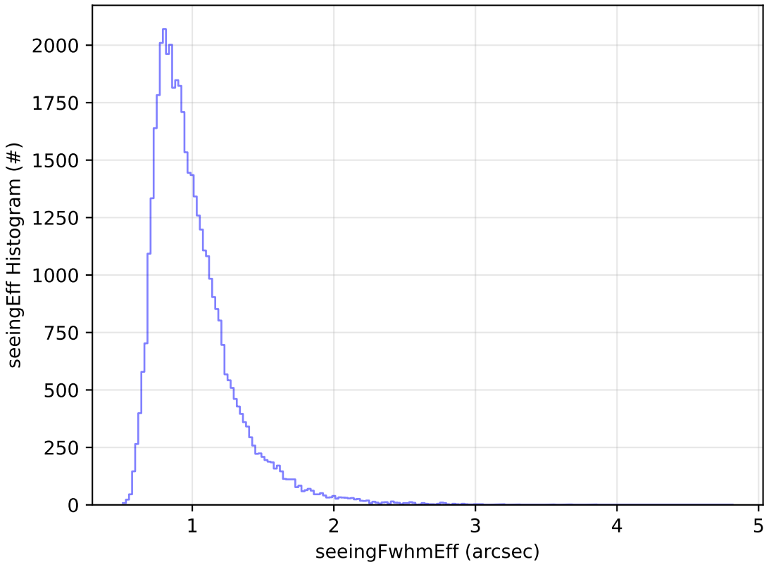
too_5_4v3.4_10yrs Yr 1 z band: seeingEff Histogram
