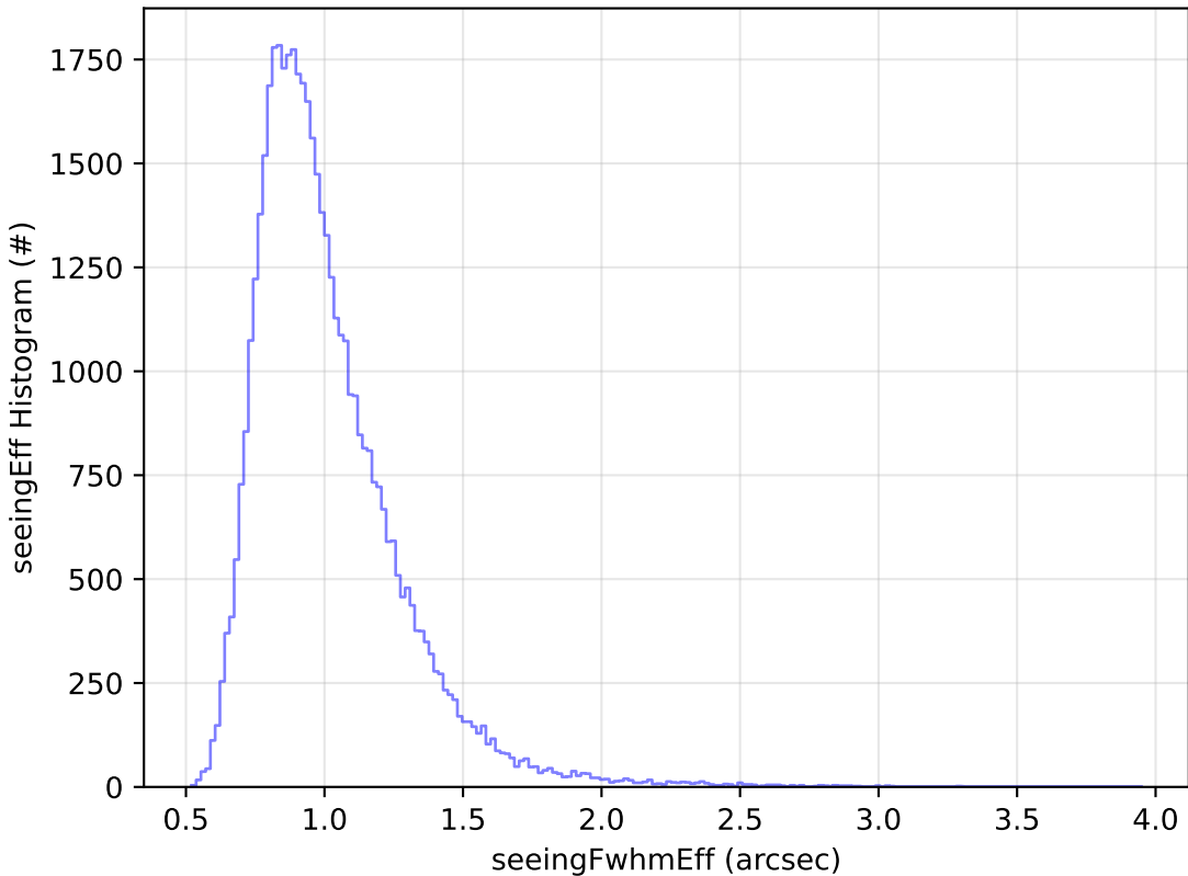
too_5_4v3.4_10yrs Yr 1 y band: seeingEff Histogram
