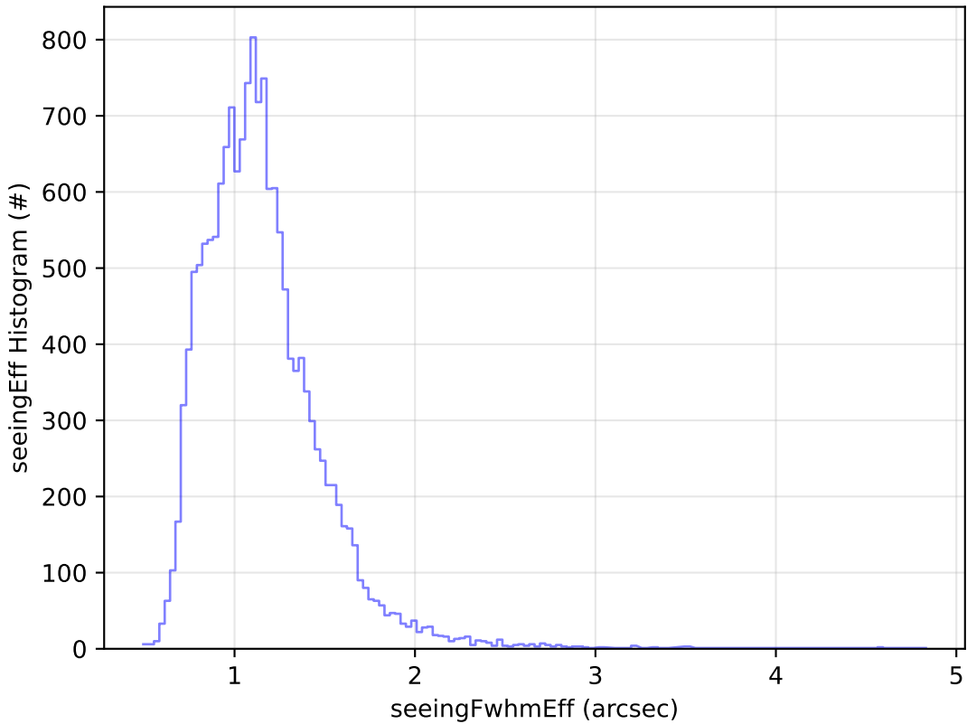
too_5_4v3.4_10yrs Yr 1 u band: seeingEff Histogram
