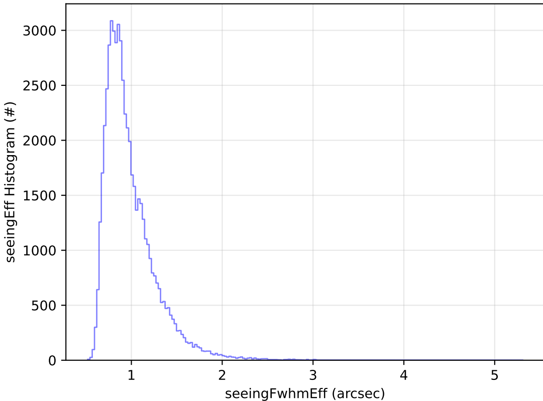
too_5_4v3.4_10yrs Yr 1 i band: seeingEff Histogram
