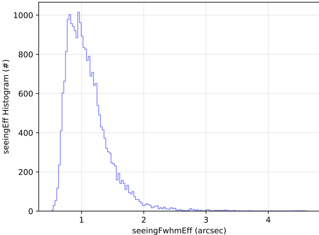
too_5_4v3.4_10yrs Yr 1 g band: seeingEff Histogram
