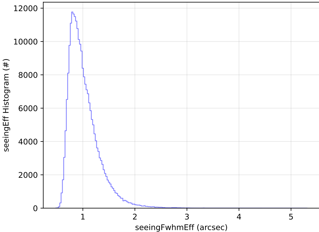
too_5_4v3.4_10yrs Yr 1 all bands: seeingEff Histogram
