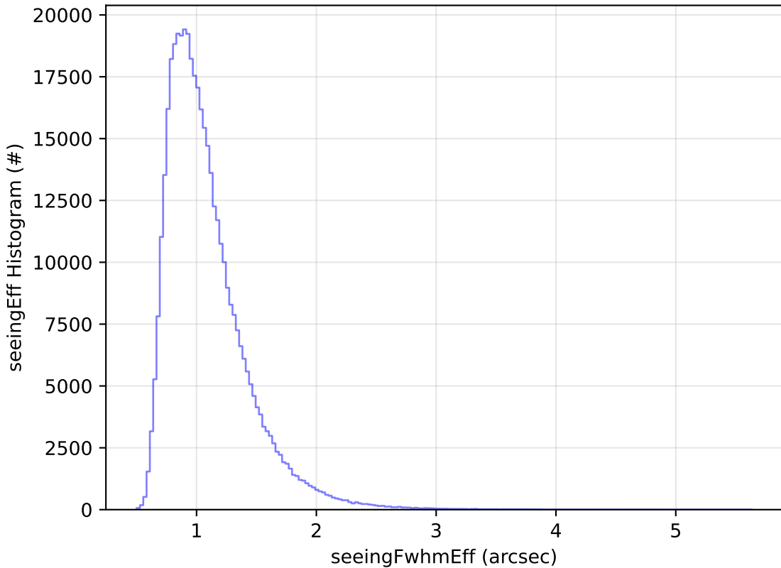
too_5_4v3.4_10yrs WFD z band: seeingEff Histogram
