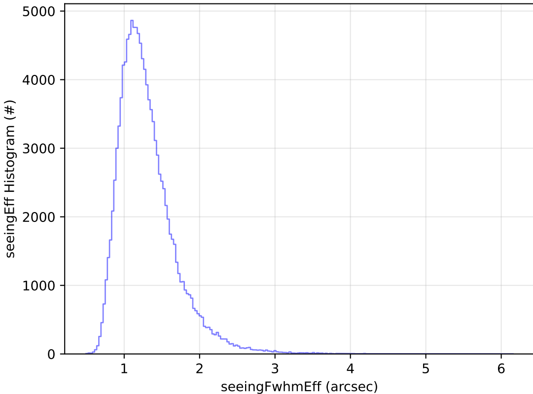
too_5_4v3.4_10yrs WFD u band: seeingEff Histogram
