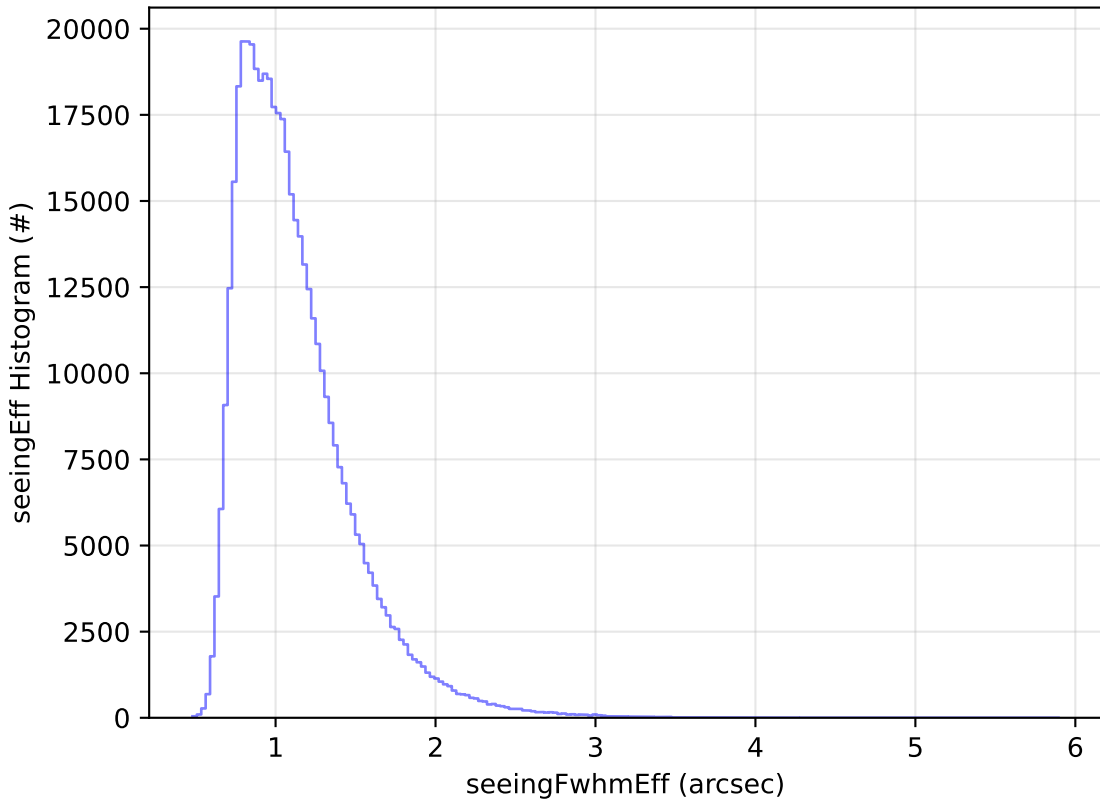
too_5_4v3.4_10yrs WFD r band: seeingEff Histogram
