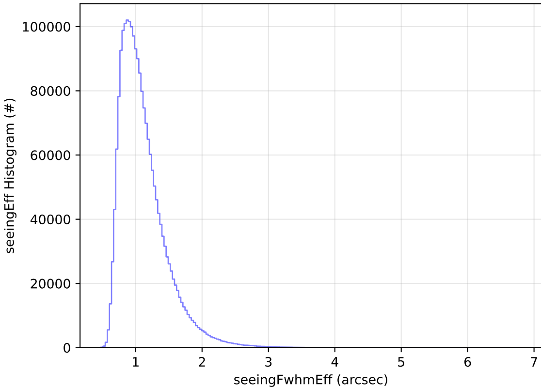
too_5_4v3.4_10yrs WFD all bands: seeingEff Histogram
