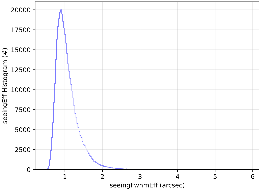
too_5_4v3.4_10yrs All sky y band: seeingEff Histogram
