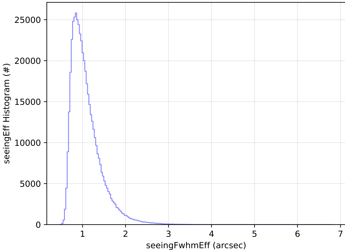
too_5_4v3.4_10yrs All sky i band: seeingEff Histogram
