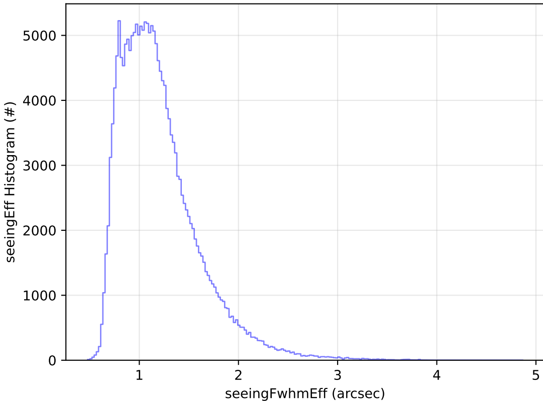
too_5_4v3.4_10yrs All sky g band: seeingEff Histogram
