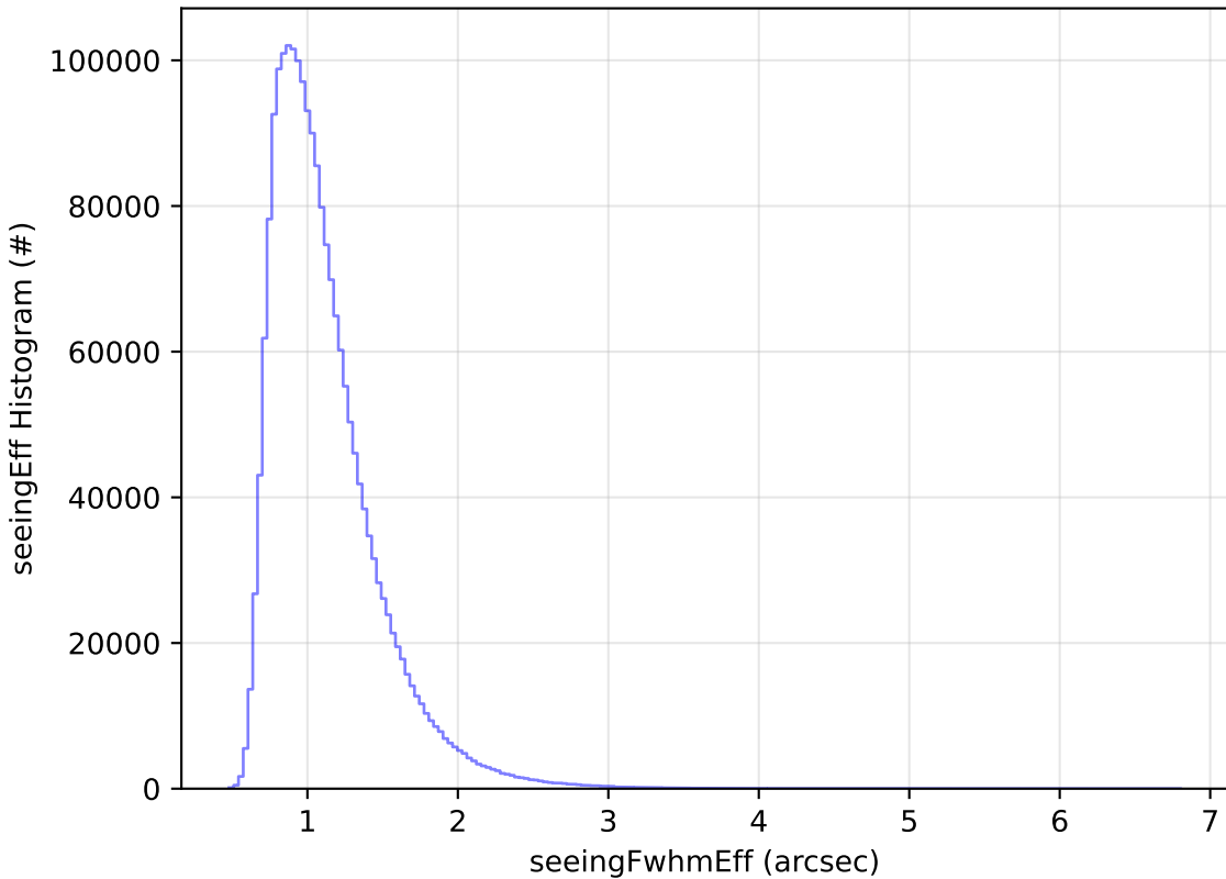
too_5_4v3.4_10yrs All sky all bands: seeingEff Histogram
