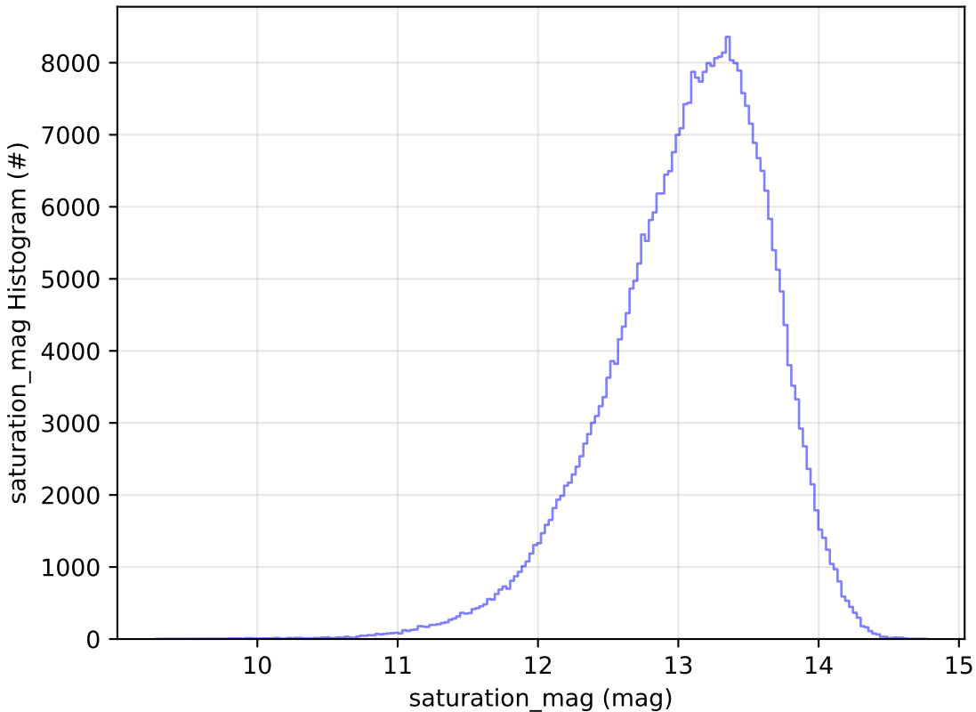
too_5_4v3.4_10yrs WFD y band: saturation_mag Histogram
