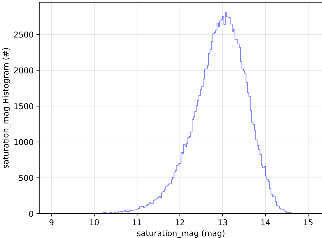
too_5_4v3.4_10yrs WFD u band: saturation_mag Histogram
