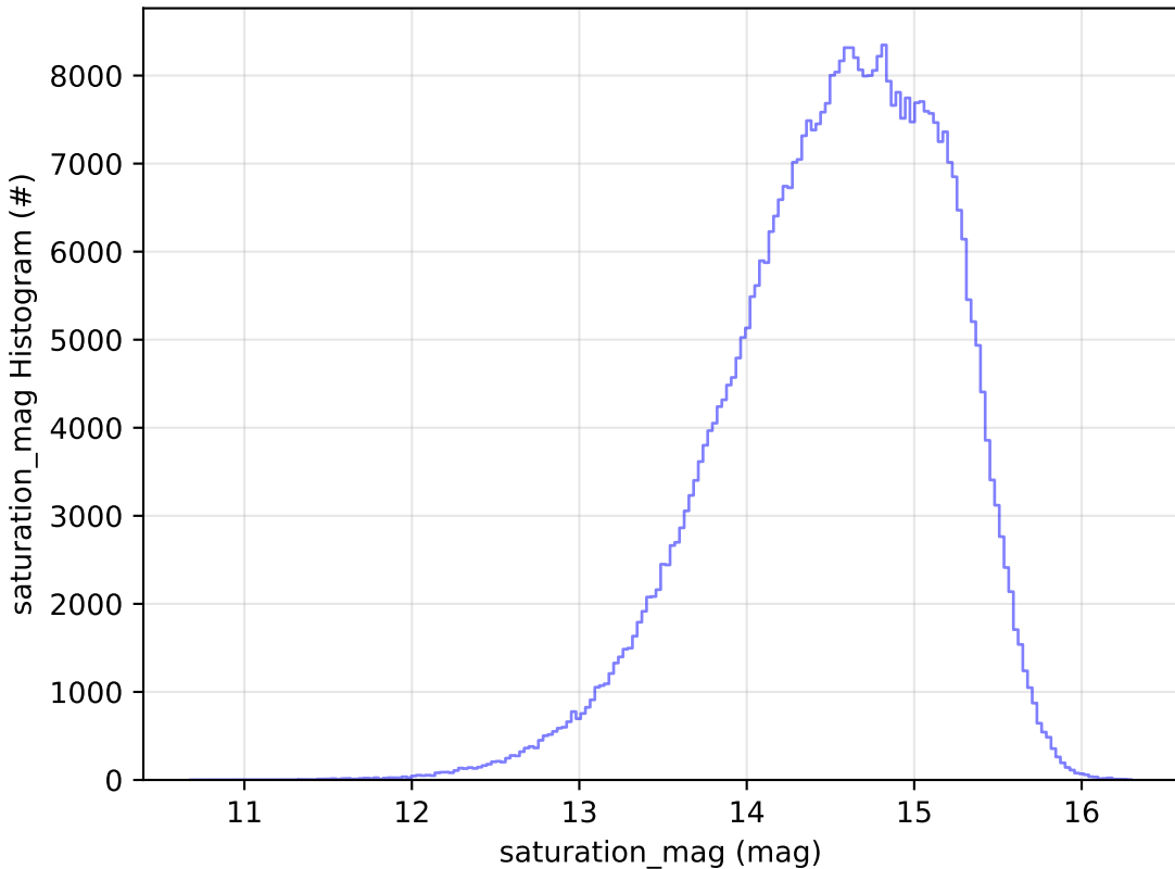
too_5_4v3.4_10yrs WFD r band: saturation_mag Histogram
