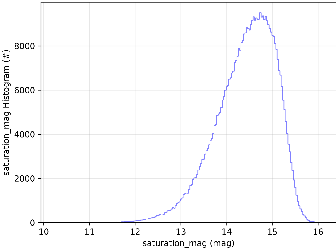
too_5_4v3.4_10yrs WFD i band: saturation_mag Histogram
