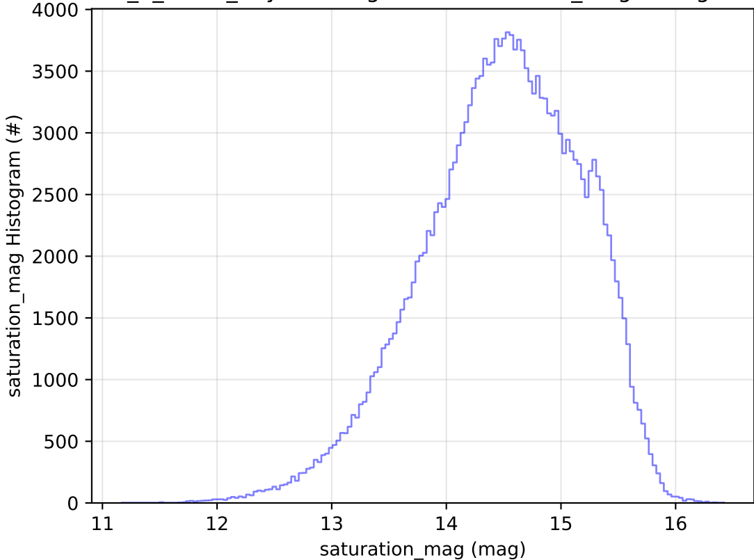
too_5_4v3.4_10yrs WFD g band: saturation_mag Histogram
