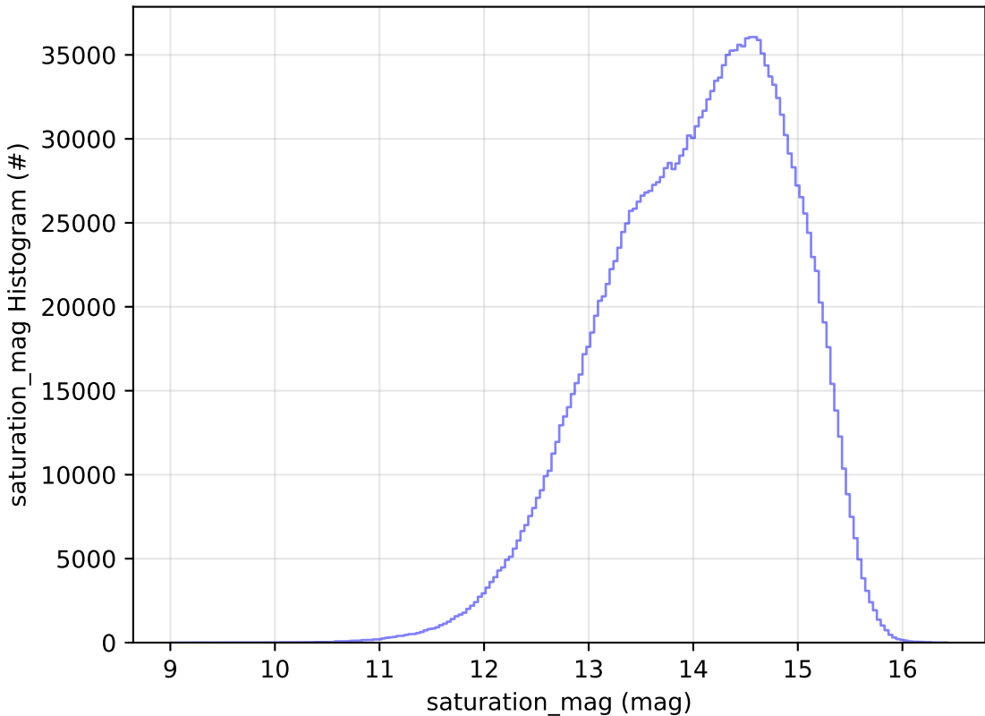
too_5_4v3.4_10yrs WFD all bands: saturation_mag Histogram
