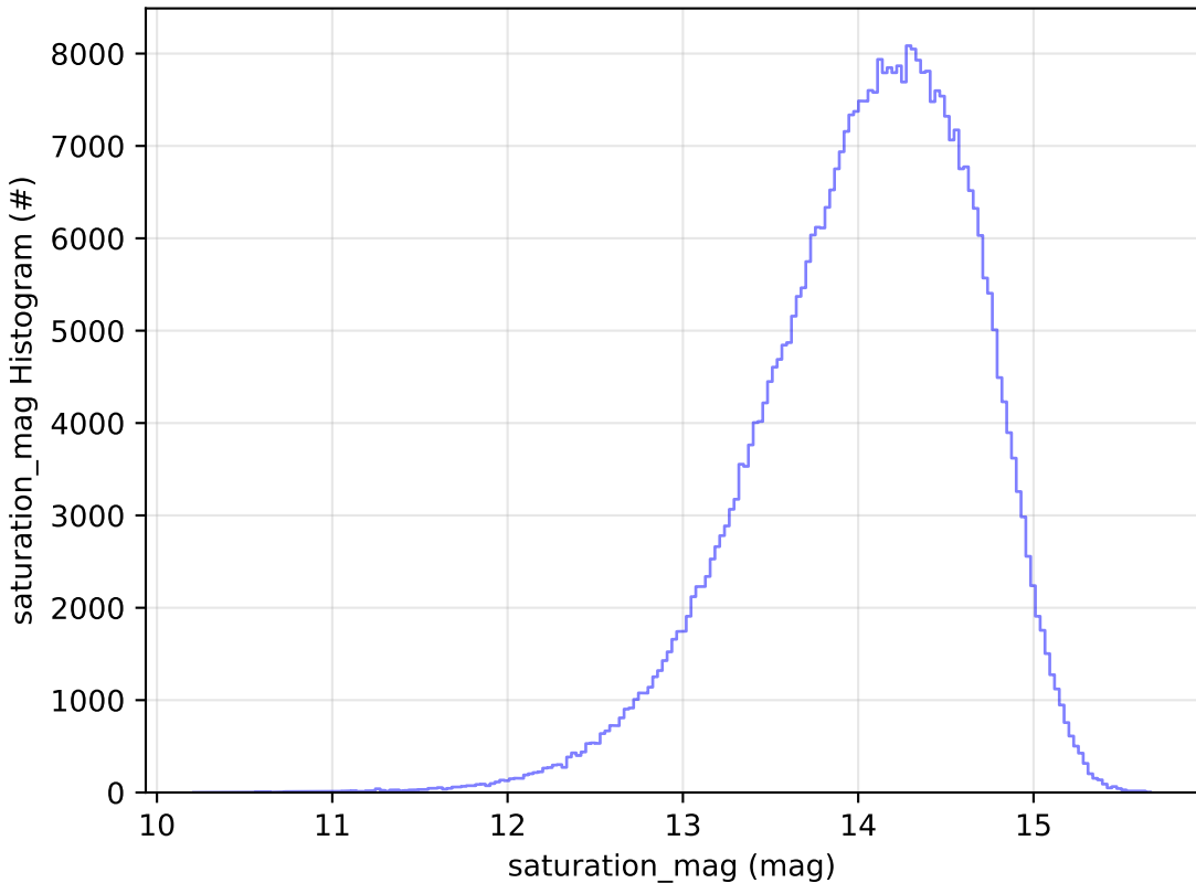
too_5_4v3.4_10yrs All sky z band: saturation_mag Histogram
