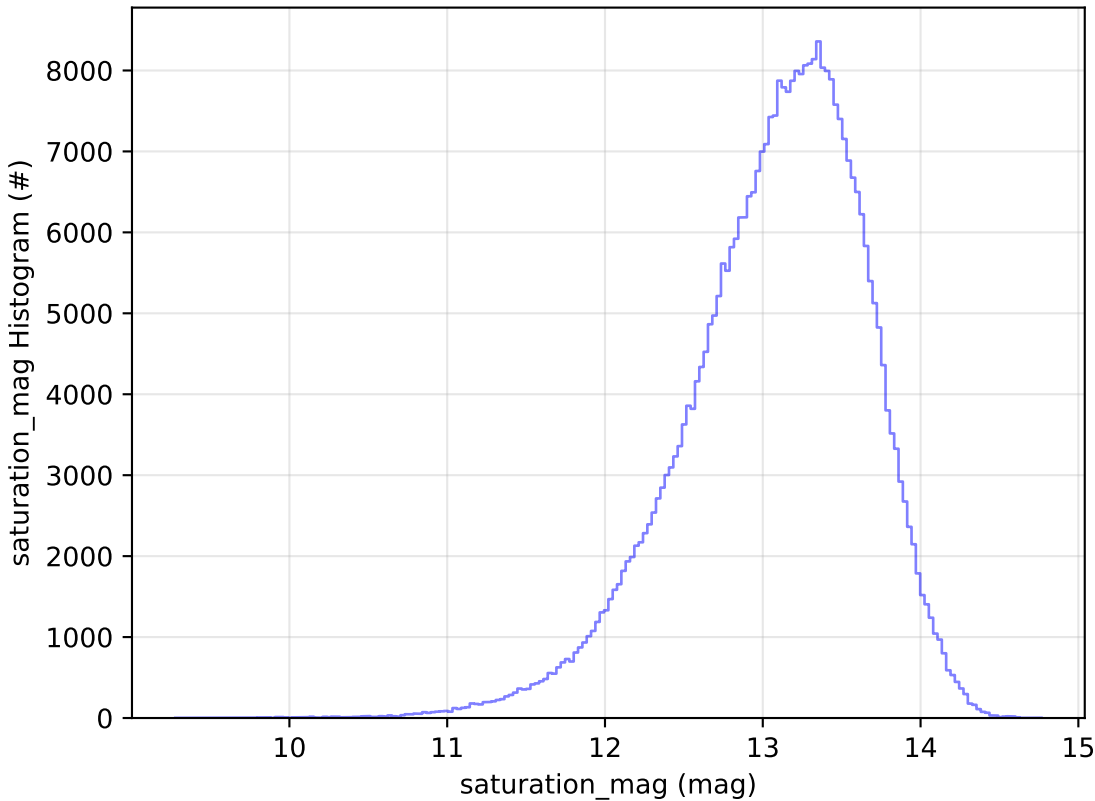
too_5_4v3.4_10yrs All sky y band: saturation_mag Histogram
