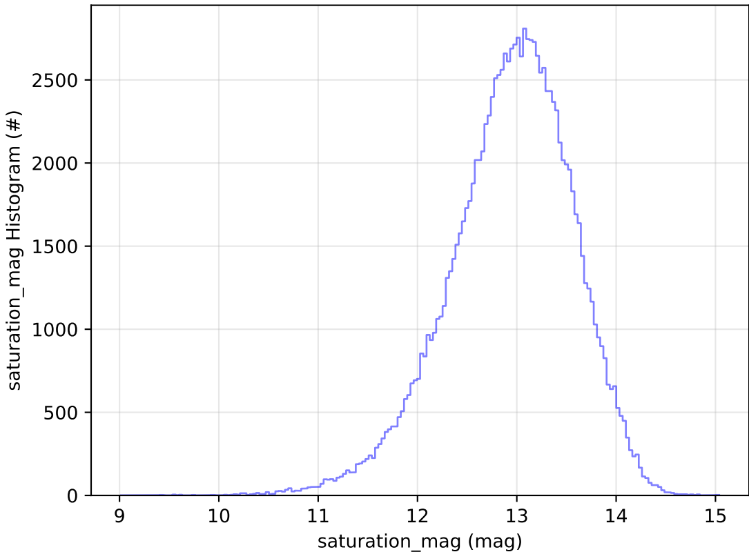
too_5_4v3.4_10yrs All sky u band: saturation_mag Histogram
