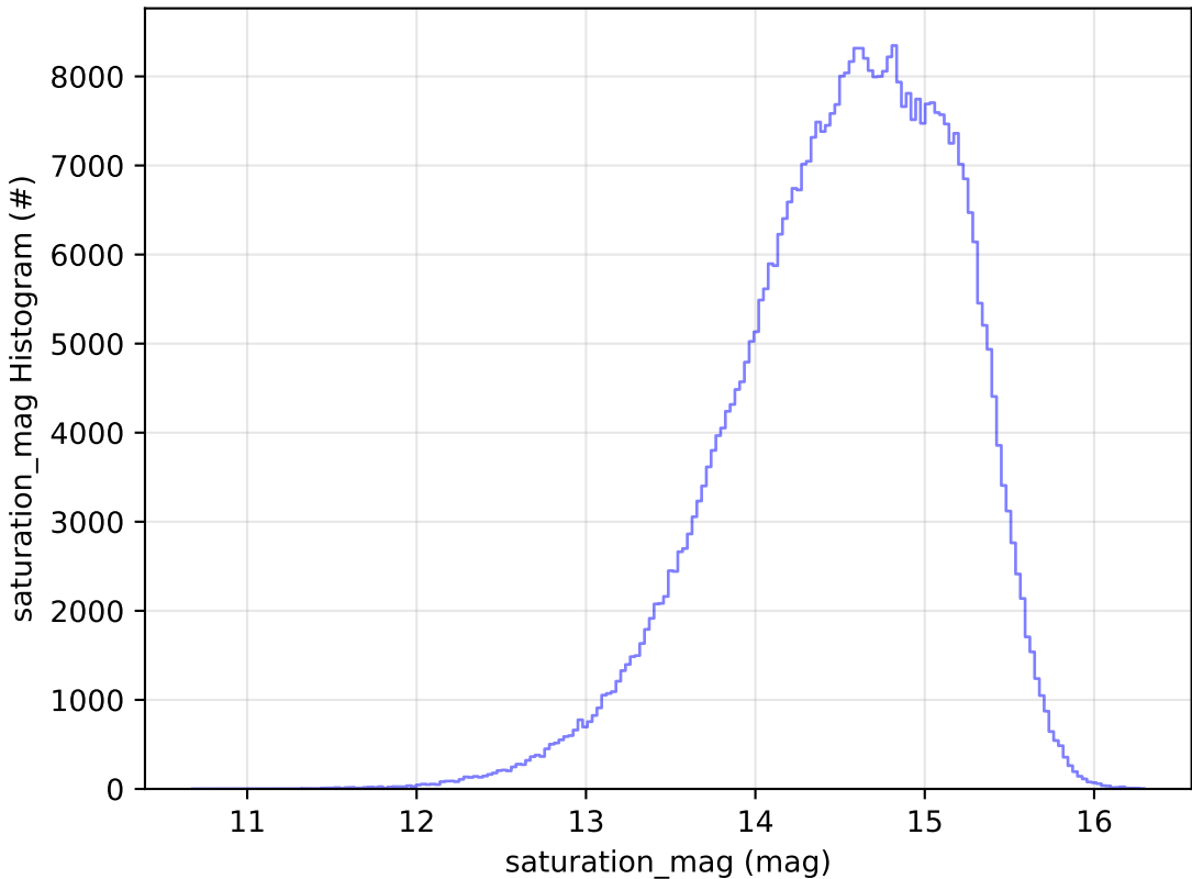
too_5_4v3.4_10yrs All sky r band: saturation_mag Histogram
