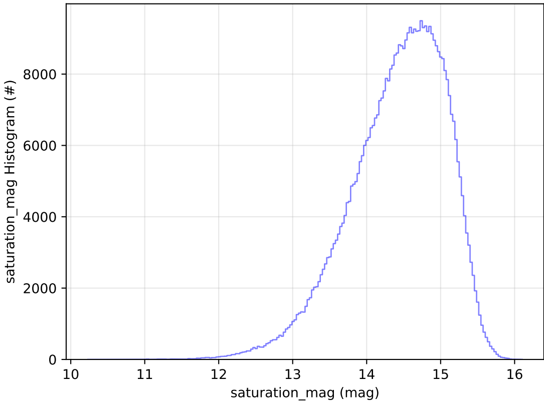
too_5_4v3.4_10yrs All sky i band: saturation_mag Histogram
