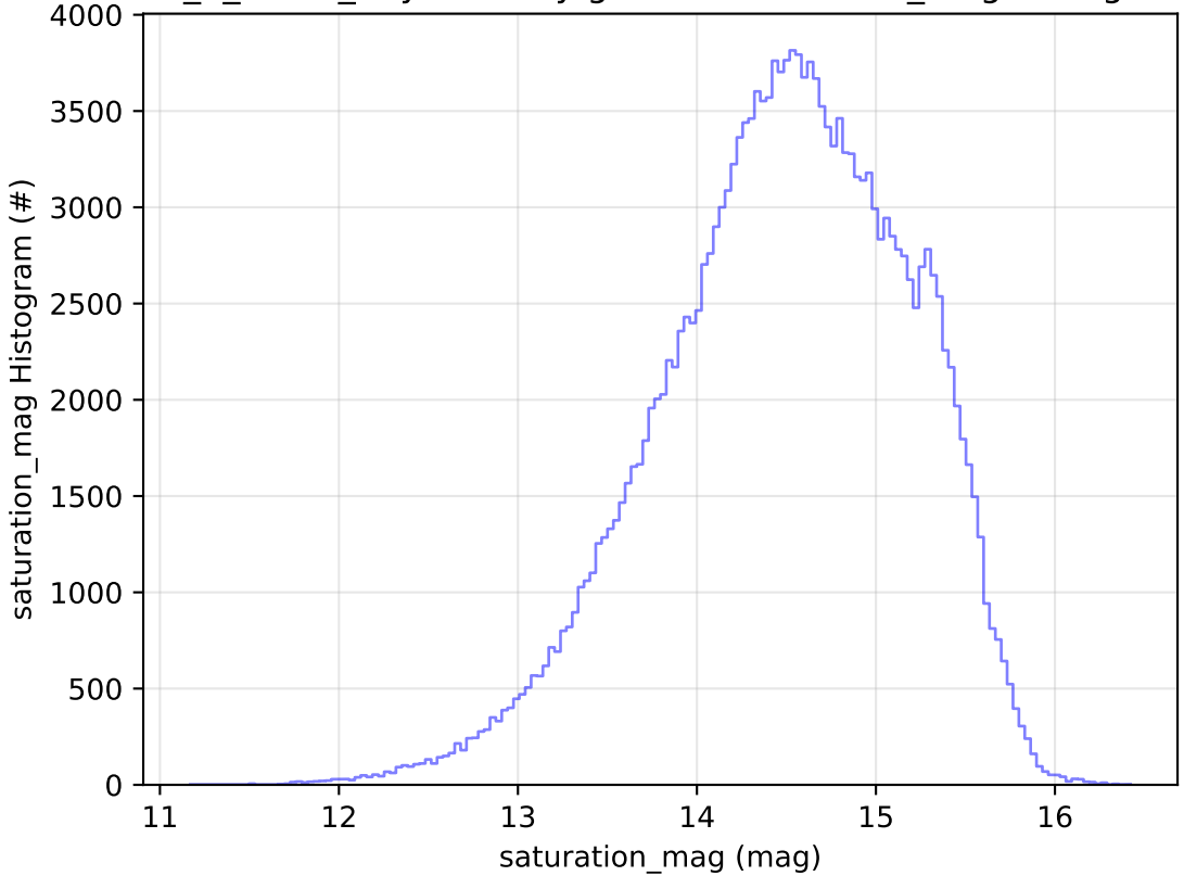
too_5_4v3.4_10yrs All sky g band: saturation_mag Histogram
