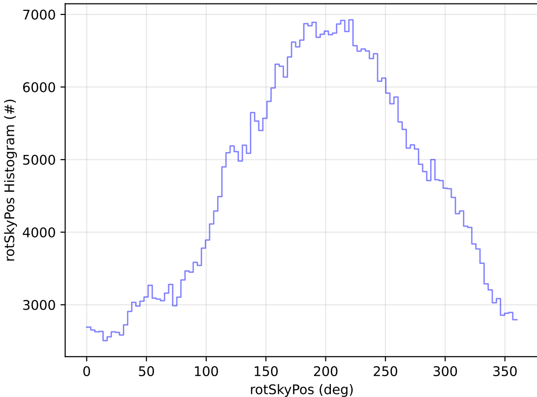
too_5_4v3.4_10yrs WFD r band: rotSkyPos Histogram
