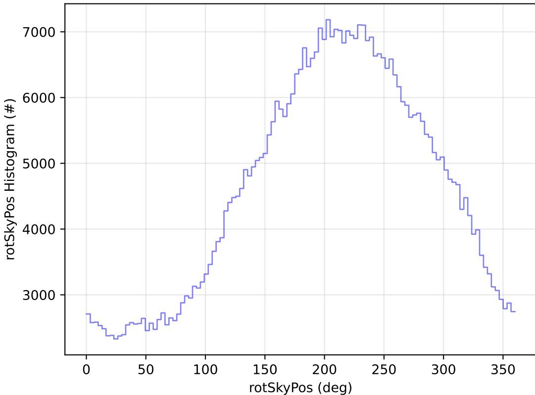
too_5_4v3.4_10yrs WFD i band: rotSkyPos Histogram
