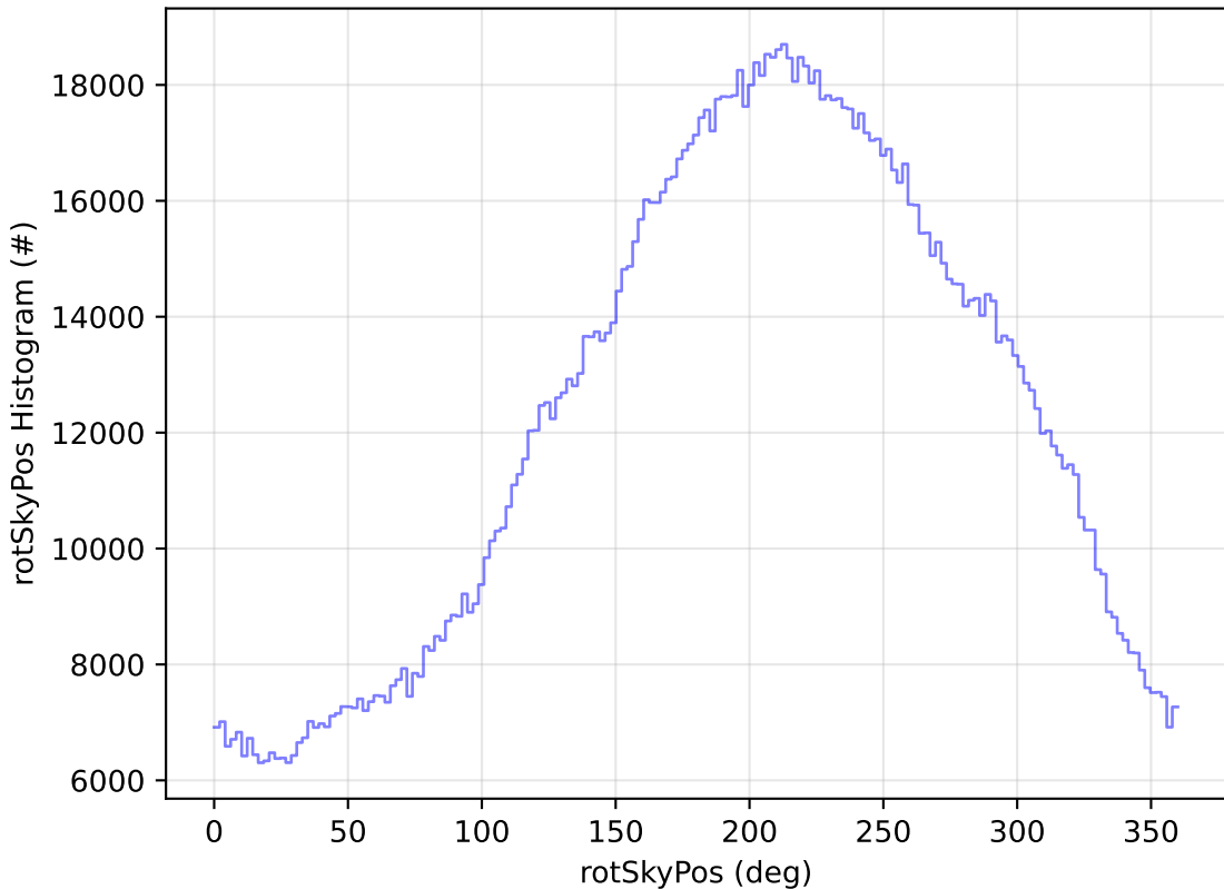
too_5_4v3.4_10yrs WFD all bands: rotSkyPos Histogram
