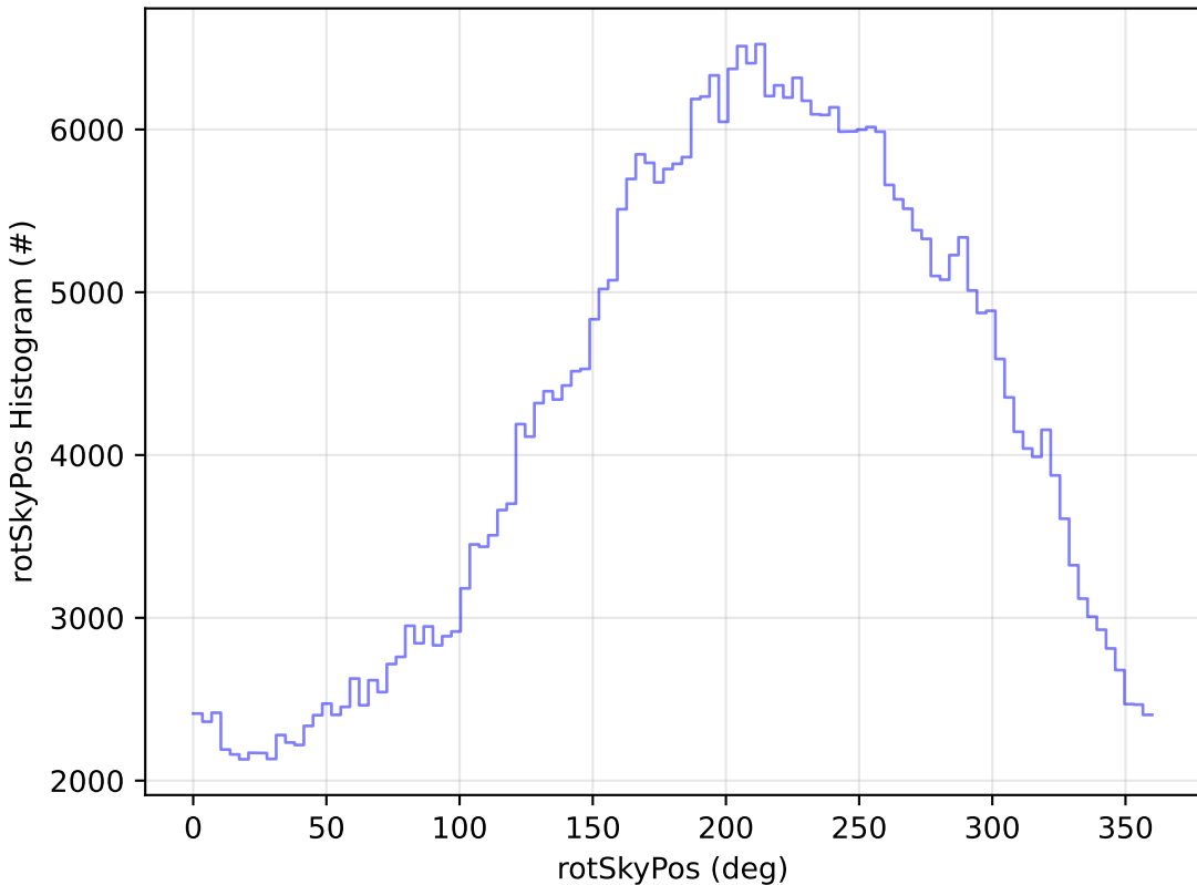
too_5_4v3.4_10yrs All sky z band: rotSkyPos Histogram
