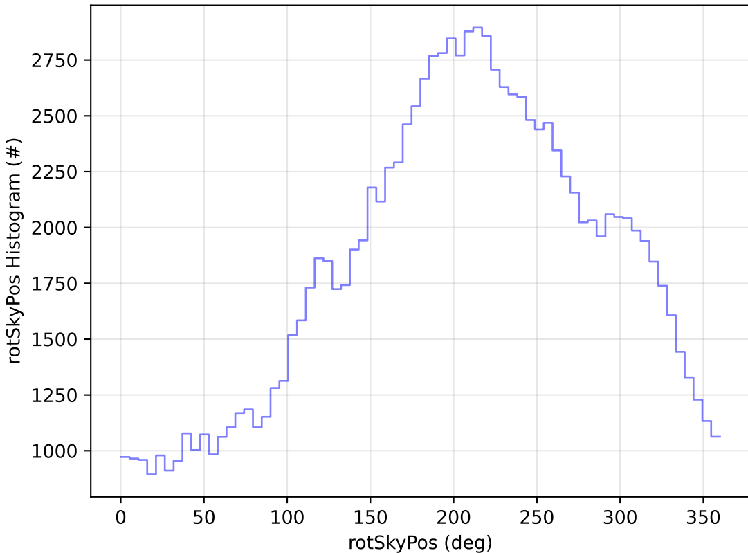
too_5_4v3.4_10yrs All sky u band: rotSkyPos Histogram
