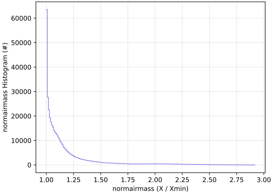
too_5_4v3.4_10yrs WFD z band: normairmass Histogram
