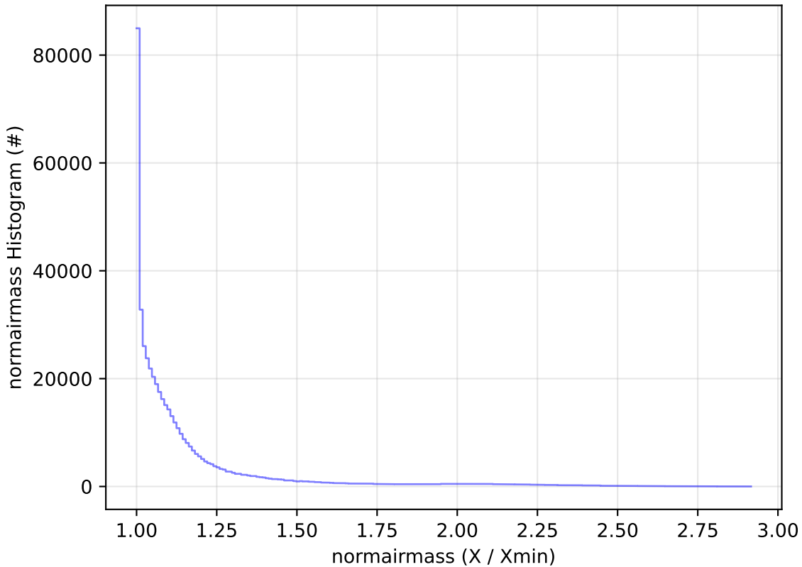
too_5_4v3.4_10yrs WFD i band: normairmass Histogram
