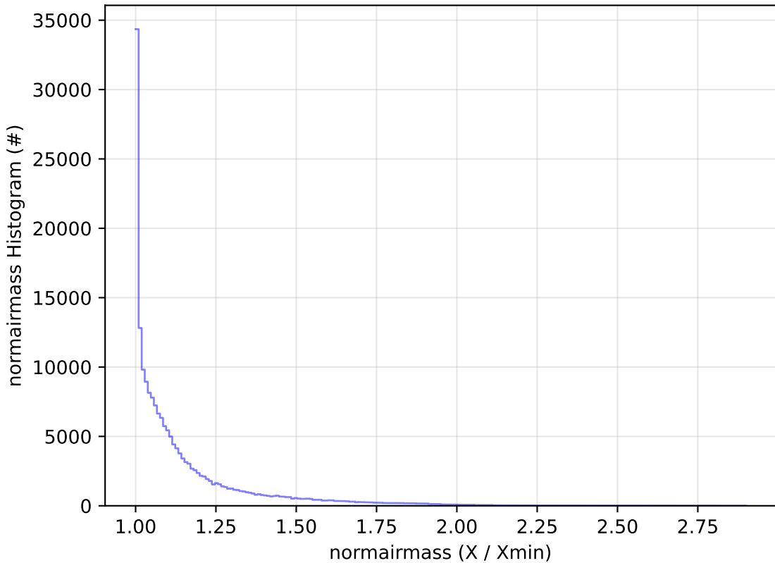
too_5_4v3.4_10yrs WFD g band: normairmass Histogram
