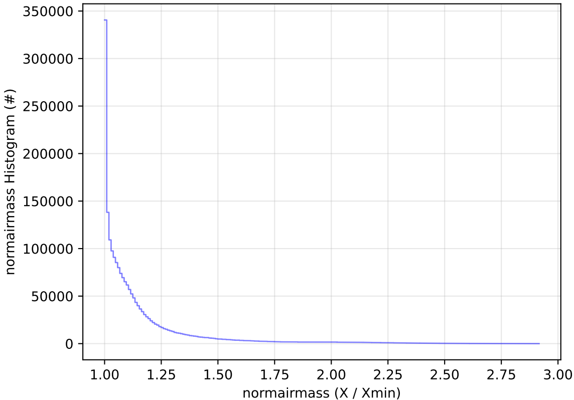
too_5_4v3.4_10yrs WFD all bands: normairmass Histogram
