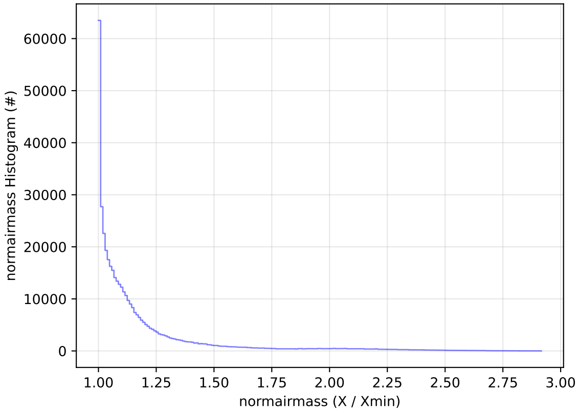
too_5_4v3.4_10yrs All sky z band: normairmass Histogram
