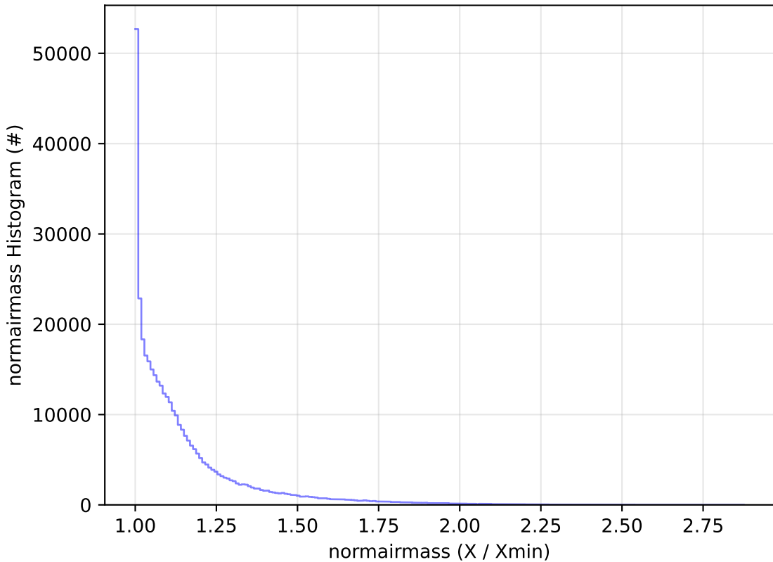
too_5_4v3.4_10yrs All sky y band: normairmass Histogram
