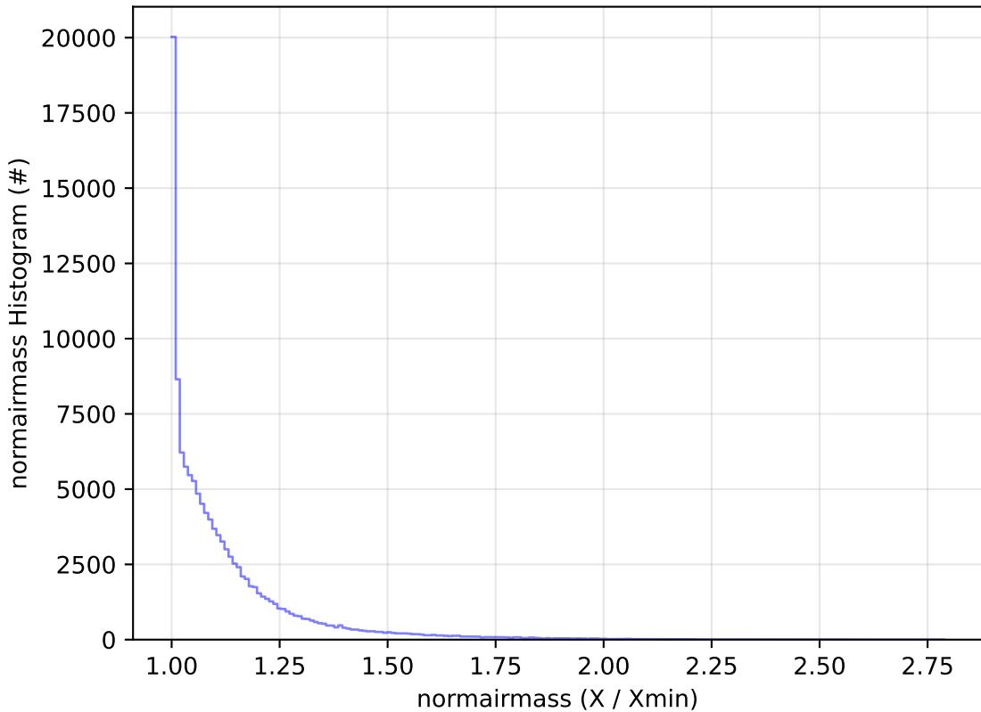
too_5_4v3.4_10yrs All sky u band: normairmass Histogram
