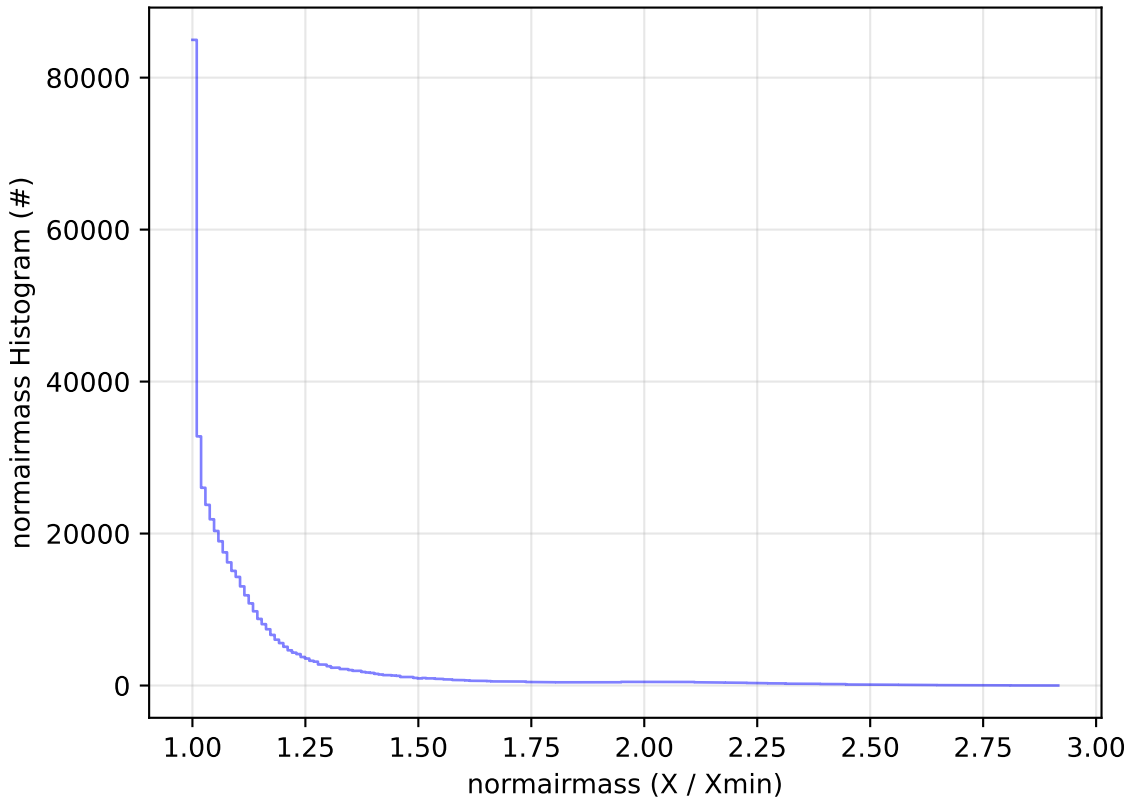
too_5_4v3.4_10yrs All sky i band: normairmass Histogram
